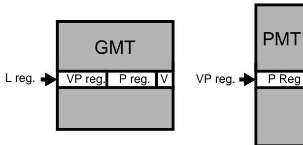
Figure 1. Tables required by the virtual-physical register organization.
