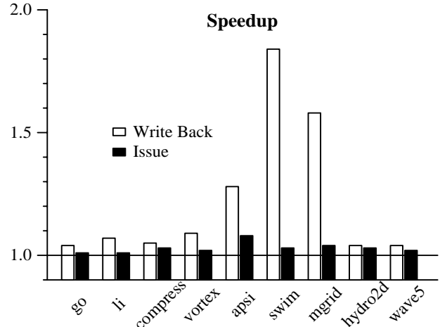
Figure 6. Write-back versus issue register allocation.
