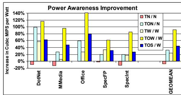
Figure 4.3 Improved power-awareness, over baseline
