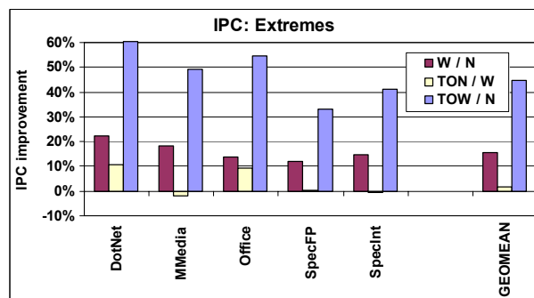
Figure 4.4 IPC improvement across configurations
