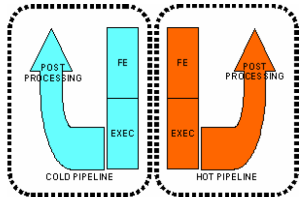
Figure 2.1 Schematic PARROT split-core march
