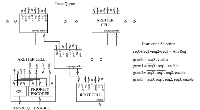
Fig. 7. Position-based selection logic.
