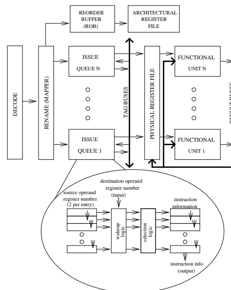
Fig. 1. Pipeline overview of the dynamic scheduling path and issue queue organization and operation.
