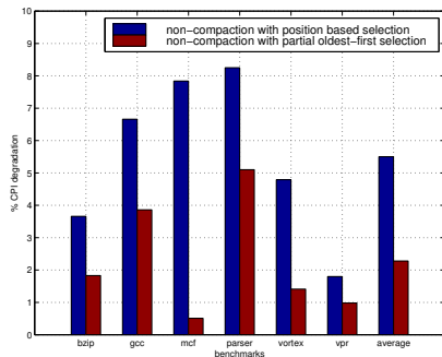
Fig. 10. CPI degradation incurred via non-compaction with position-based selection, and non-compaction with partial oldest-first selection.
