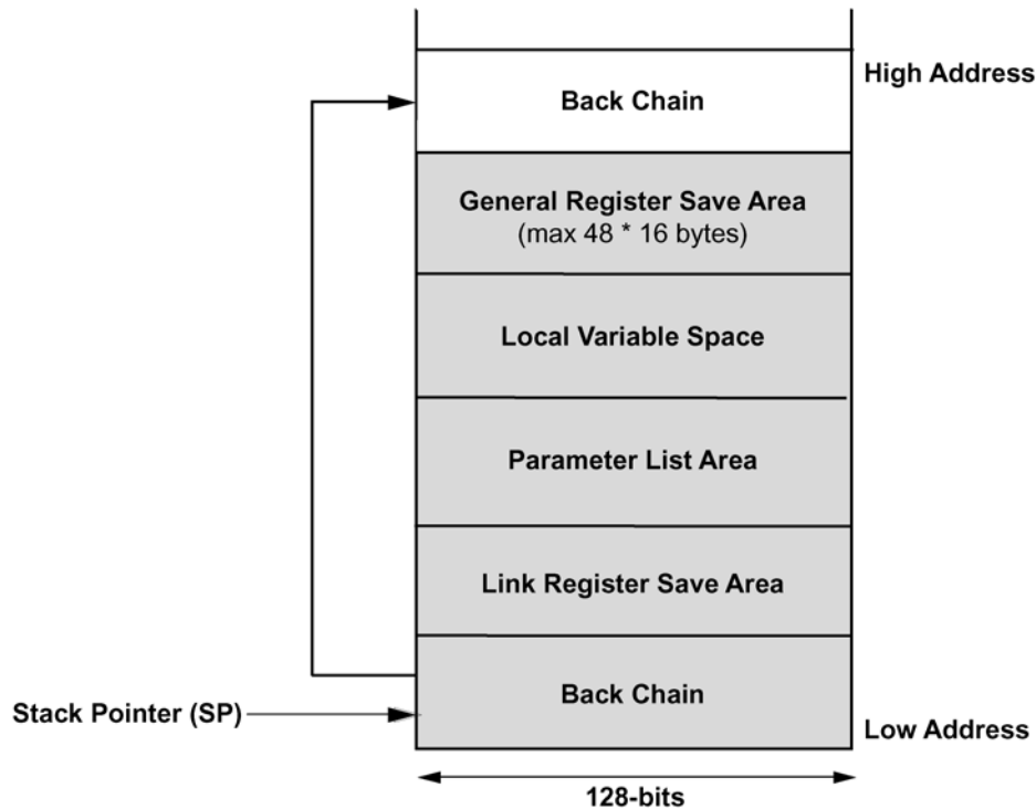
Figure 2-12: Standard Stack Frame
