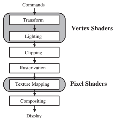
Figure 1. Graphics pipeline
